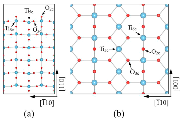
Figure 1. (a) Side and (b) top view of the periodic six-layer slab with a (4 \times 2) surface supercell that is used to model the rutile \text{TiO}_2(110) surface. 5-fold coordinated \text{Ti}_{5c} , 6-fold coordinated \text{Ti}_{6c} , 2-fold coordinated bridging \text{O}_{2c} , and 3-fold coordinated in-plane \text{O}_{3c} atoms are indicated. Light blue and red balls represent Ti and O atoms, respectively.
